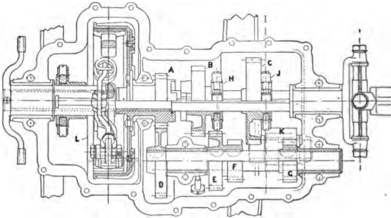
FIG. 258.--Transmission and Clutch of the Columbia Light Car. A, spur gear on the clutch shaft; B and C, spurs on the squared second shaft, the first shifted by fork hung at H, by lever, H (last figure), the second by fork at J by lever, J. D, E, F, G, three-speed pinions keyed to countershaft; K, pinion giving reverse when in mesh with C and G; L, clutch.
